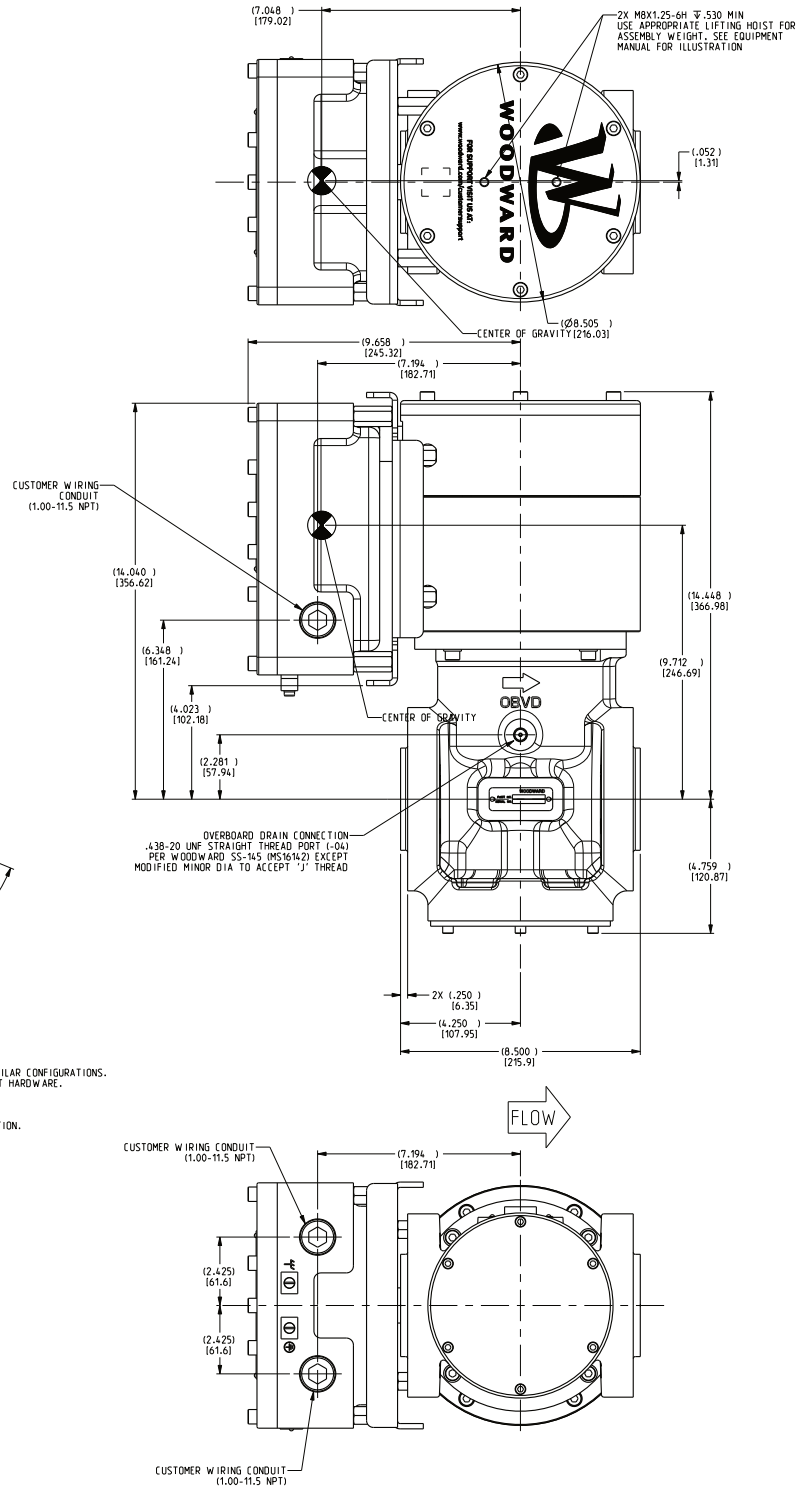
Figure 3. GS50 Outline Drawing A
